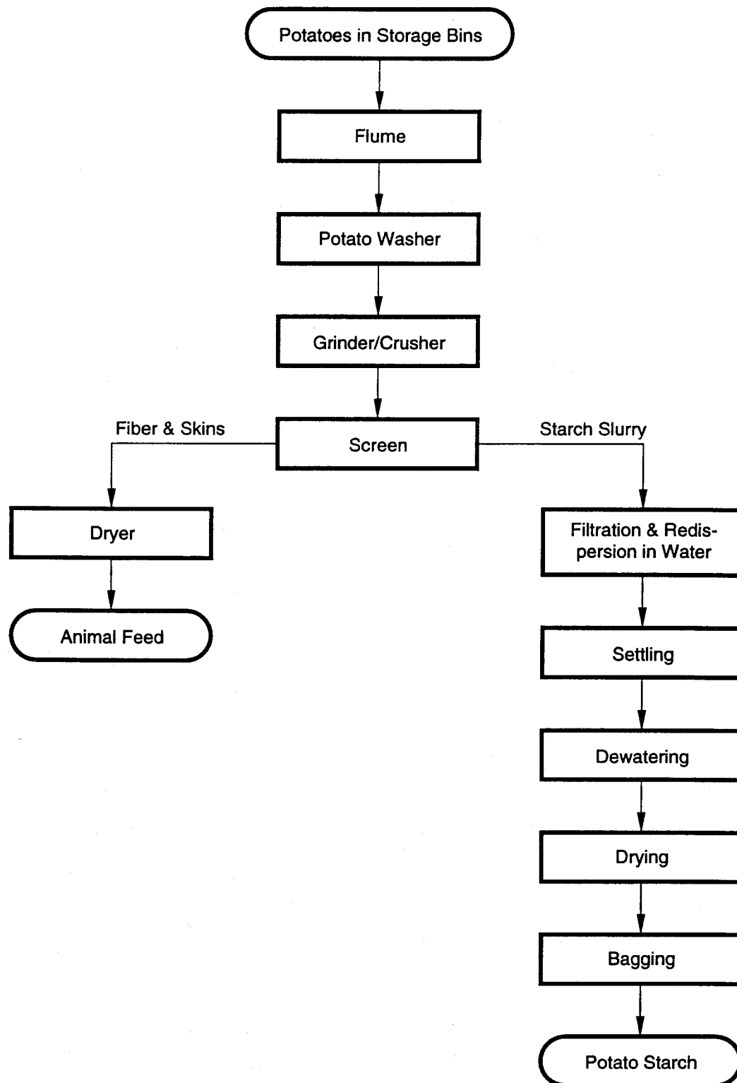
Figure 2-5. Potato starch process.
