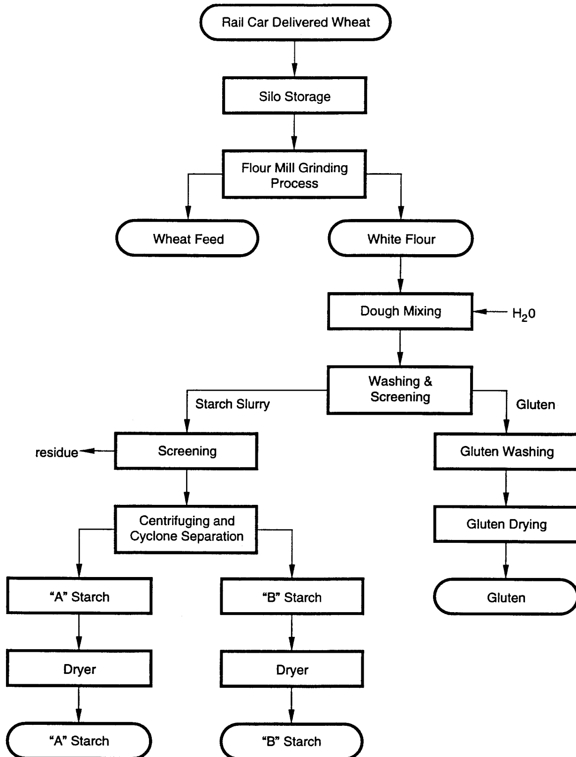
Figure 2-4. Wheat starch production process.
